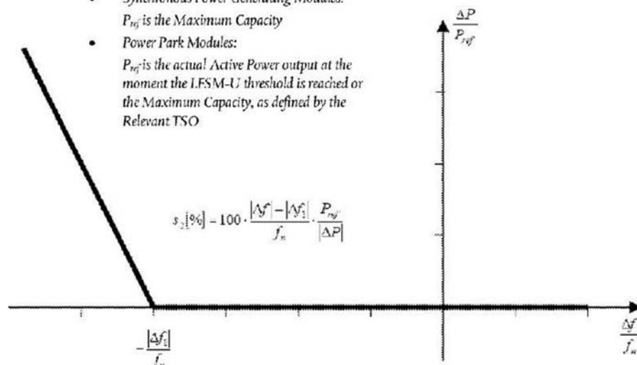
Figure 27 - LFSM-U characteristic
