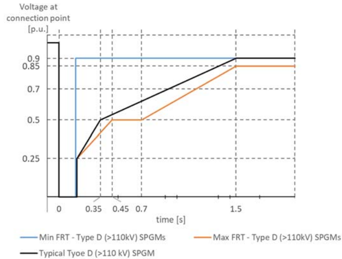
Figure 38 - Min and max possible FRT requirement, and typical response of type D SPGM connected at or above 110kV
