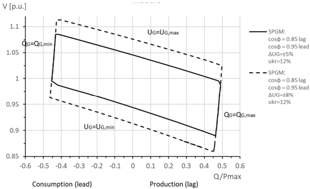
Figure 43 - Typical SPGM voltage-var characteristic
