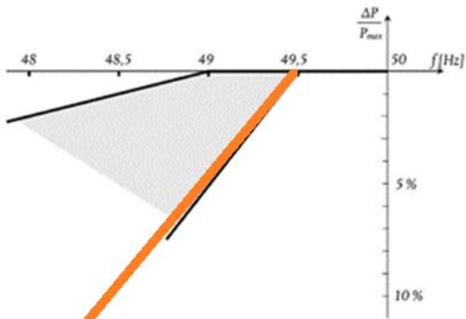
Figure 30 - Recommendation for parameter Admissible active power reduction from max. output with falling frequency
