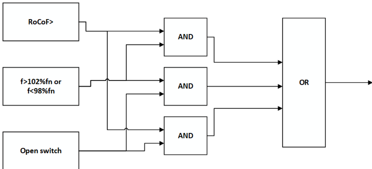
Figure 20 - Loss of Mains algorithm 2 of 3
