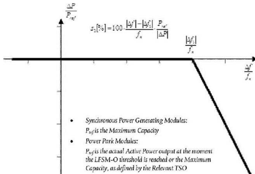
Figure 26 - LFSM-O characteristic
