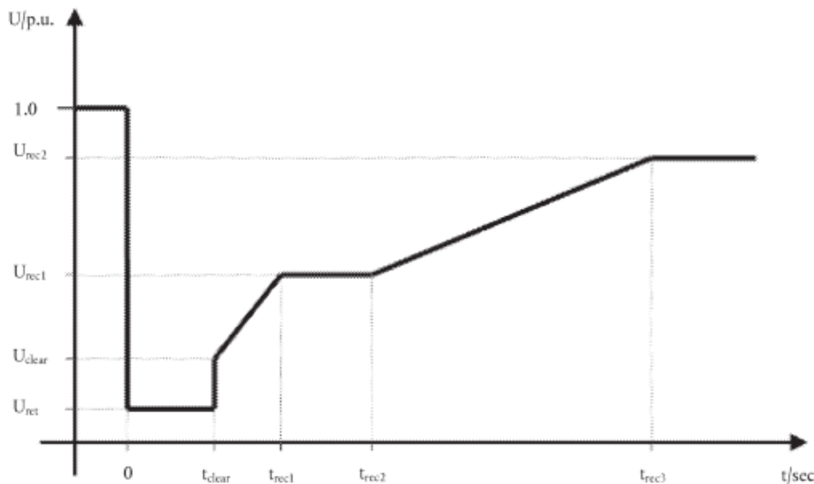
Figure 34 - Generic FRT voltage-against time profile ([1]Figure 3)
