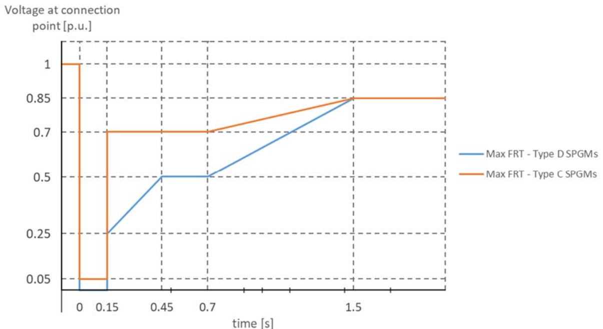
Figure 14 - Maximum FRT requirements for type C and D SPGMs
