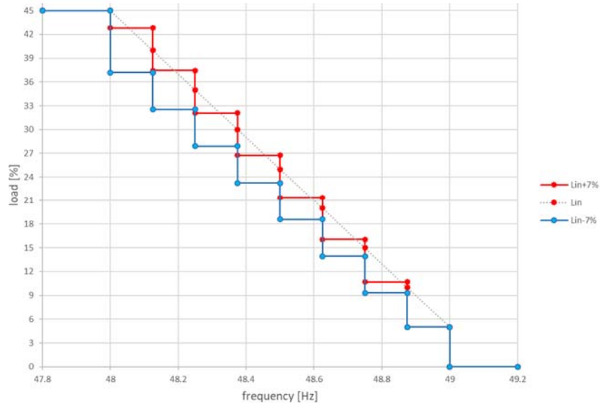
Figure 57 - Graphically presentation of the conditions for LFDD schema
