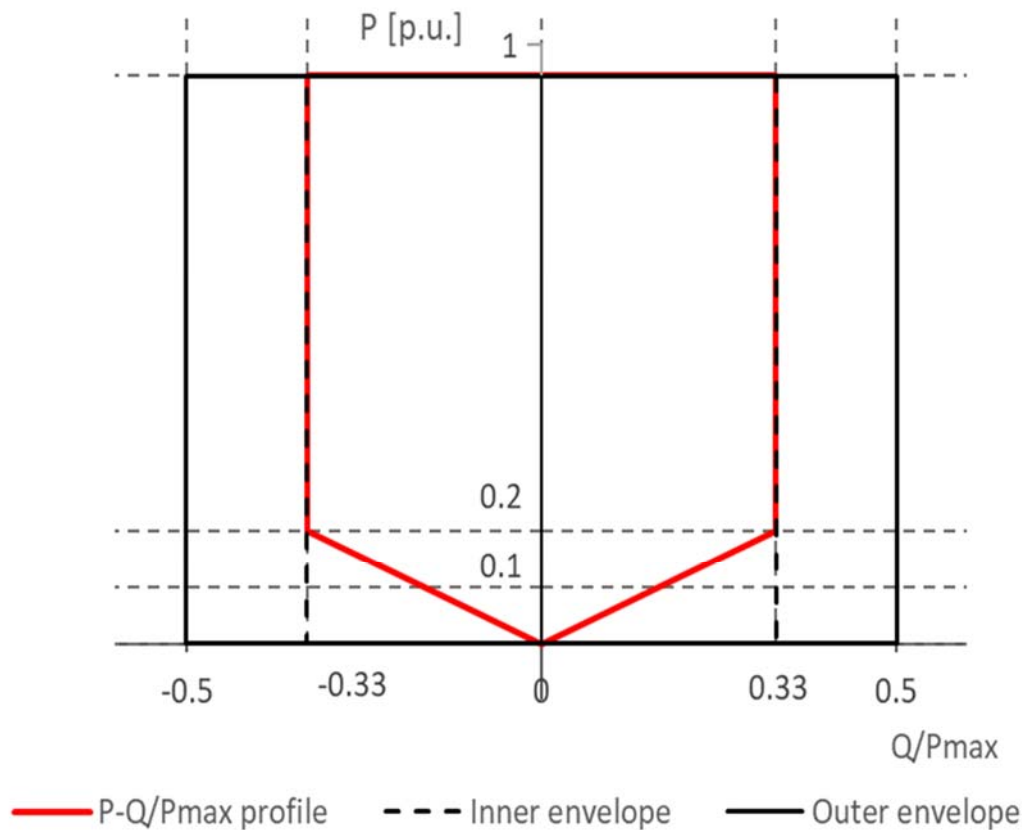
Figure 50 - Proposed P-Q/Pmax characteristics for PPMs Voltage/Reactive Power Control
