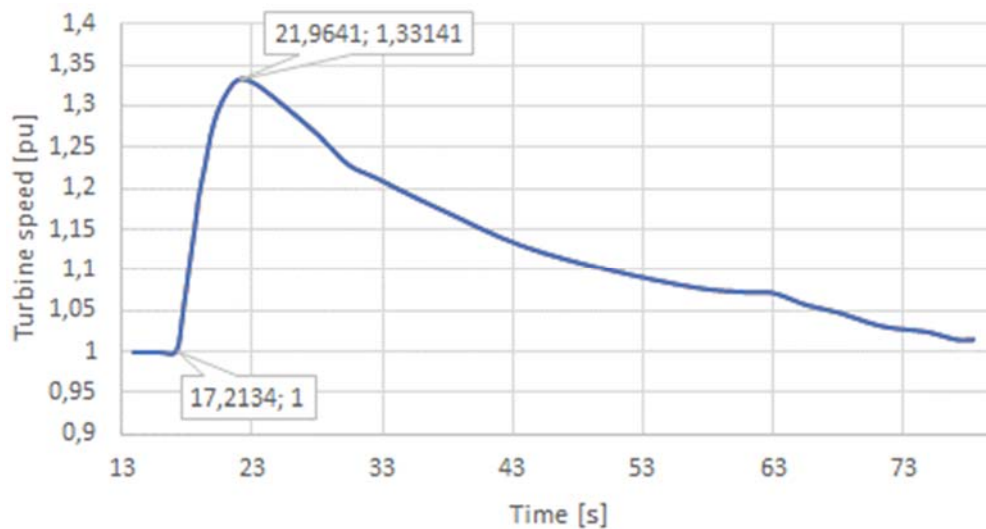
Figure 18 - Load rejection on typical HPP
