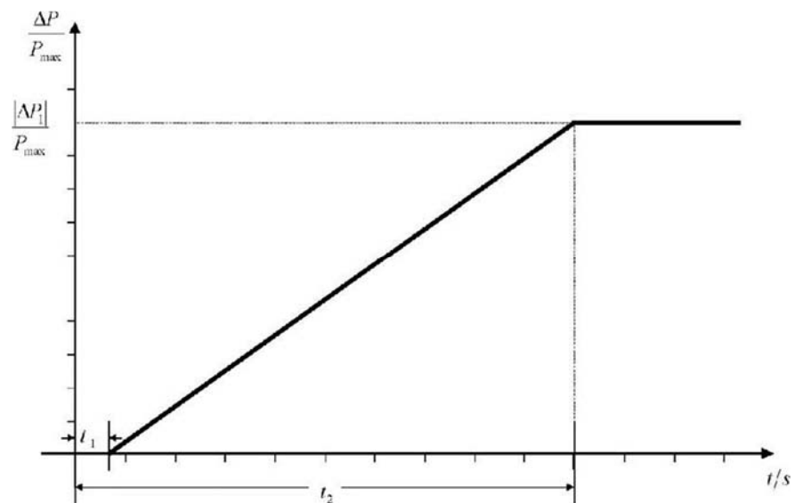
Figure 22 - FCR response characteristic
