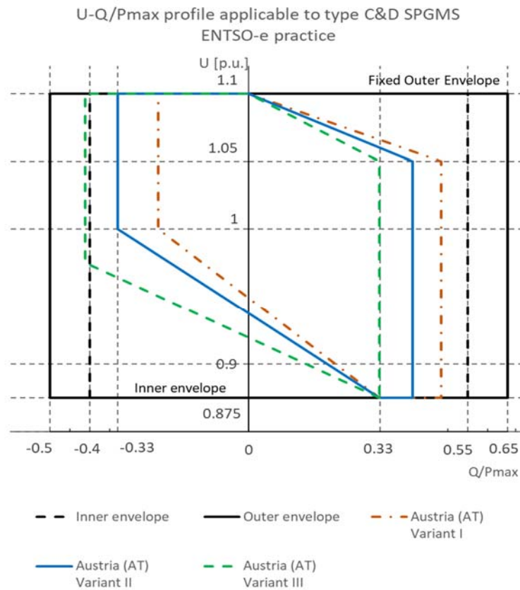
Figure 65 – Reactive power capability requirement applicable to type C & D SPGMS and PPMs implemented in Austria
