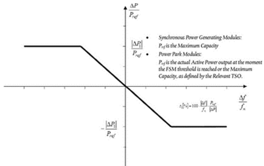
Figure 21 - FSM characteristic
