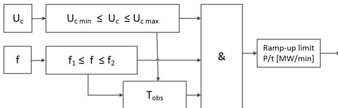
Figure 31 - Principle for automatic reconnection
