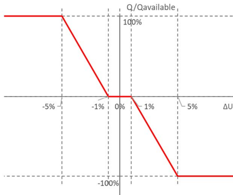
Figure 52 - Illustration of reactive power droop and voltage deadband
