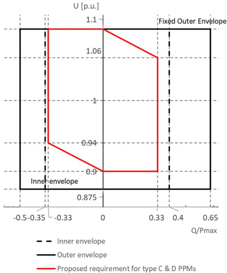
Figure 47 - Proposed U-Q/Pmax requirement for type C and D PPMs
