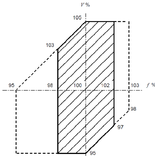
Figure 33 - Voltage and frequency limits for steam or gas turbine driven SPGMs with rated output at or above 10 MVA according to IEC 60034-1 standard
