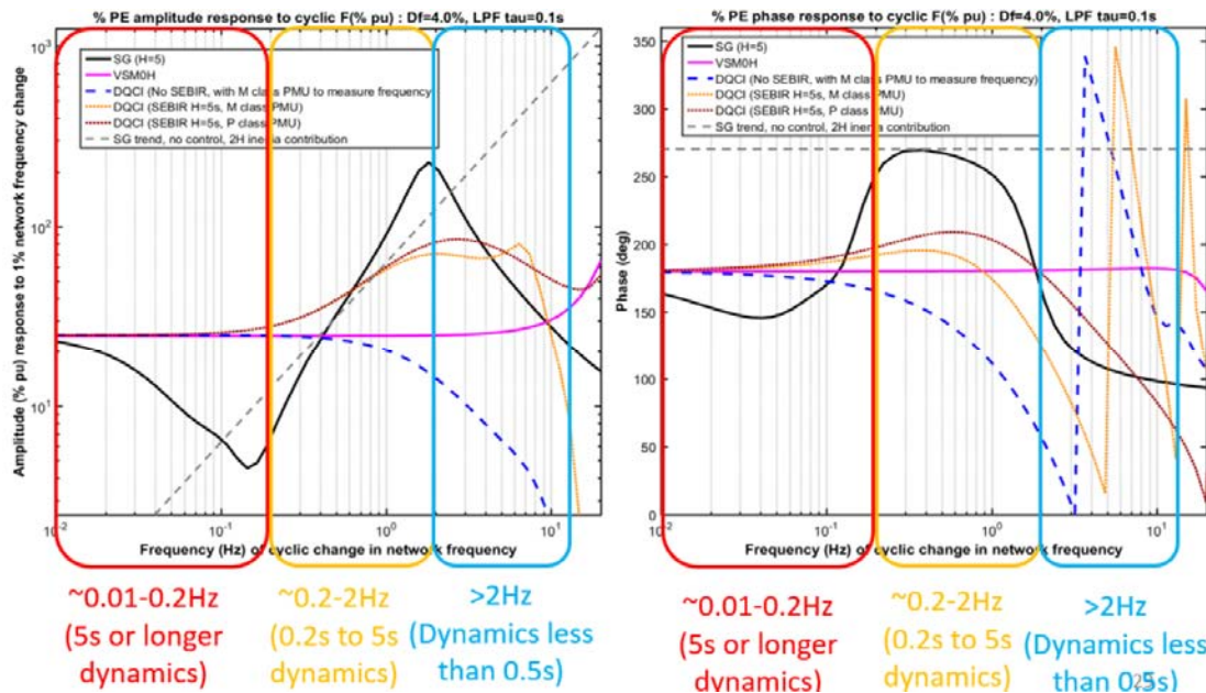
Figure 54 - Response of DQCI SEBIR controlled converters compared to SPGM's inertial response (Source: [17] Figure 2)
