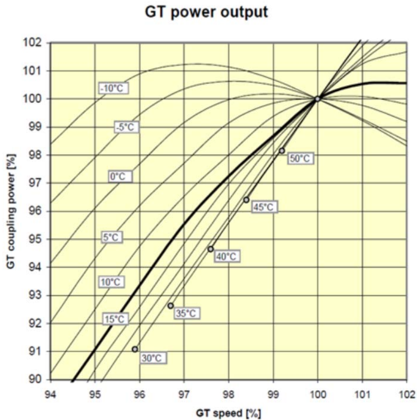
Figure 29 - Gas turbine power output
