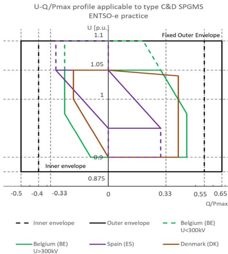
Figure 66 – Reactive power capability requirement applicable to type C & D SPGMS implemented in Belgium, Denmark and Spain 23
