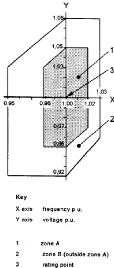
Figure 31 - Voltage and frequency limits for AC generators according to IEC 60034-1 standard
