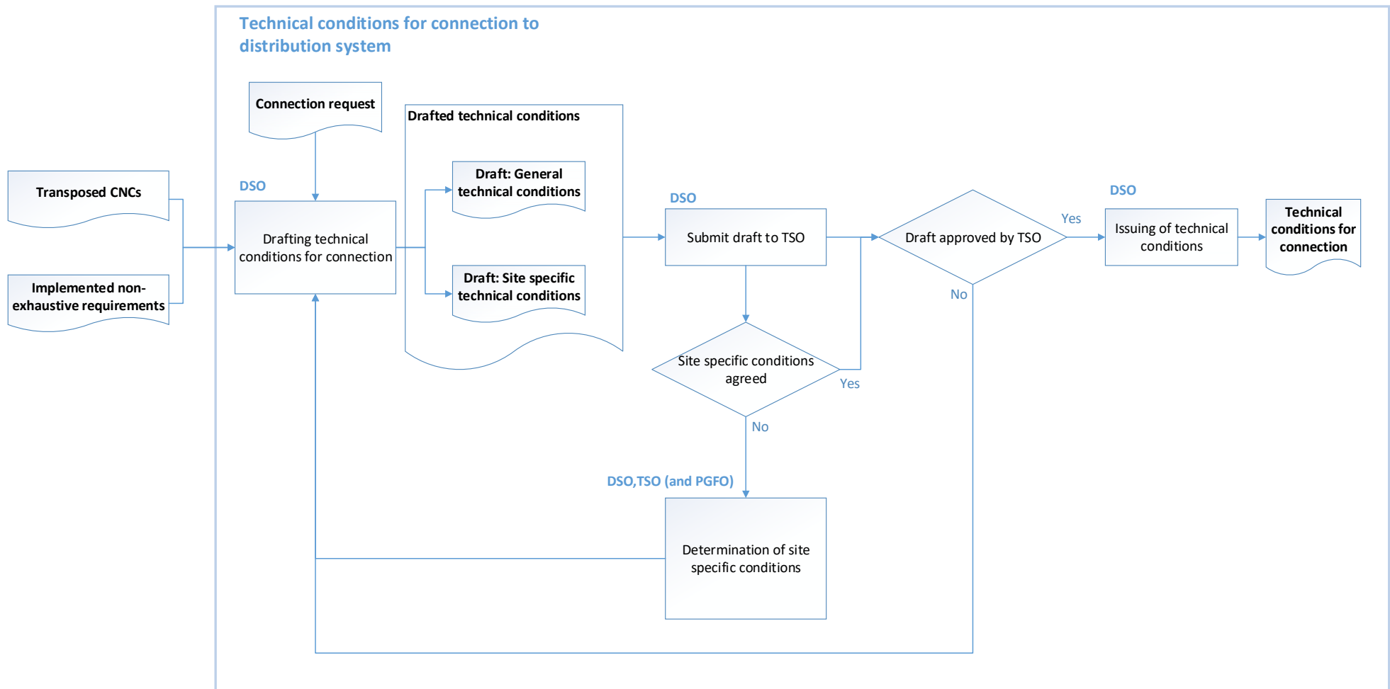
Figure 74 - DSO issues technical conditions for connection
