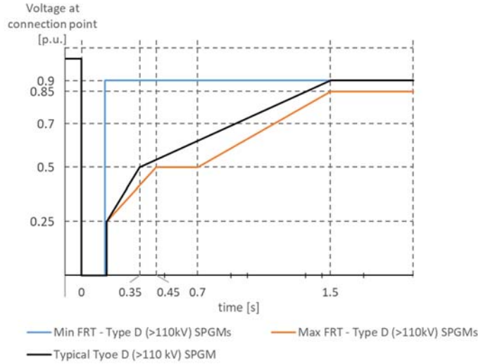
Figure 37 - Min and max possible FRT requirement, and typical response of type D SPGM connected at or above 110kV
