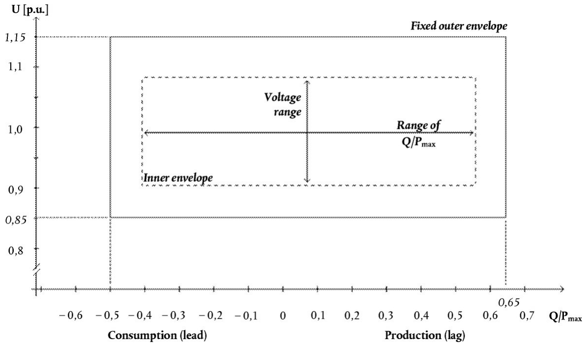
Figure 7: U-Q/Pmax-profile of a DC-connected power park module at the connection point. The diagram represents boundaries of a U-Q/Pmax-profile of the voltage at the connection point[s], expressed by the ratio of its actual value to its reference 1 pu value in per unit, against the ratio of the reactive power (Q) to the maximum capacity (Pmax). The position, size and shape of the inner envelope are indicative and other than rectangular may be used within the inner envelope. For profile shapes other than rectangular, the voltage range represents the highest and lowest voltage points. Such a profile would not give rise to the full reactive power range being available across the range of steady-state voltages.
