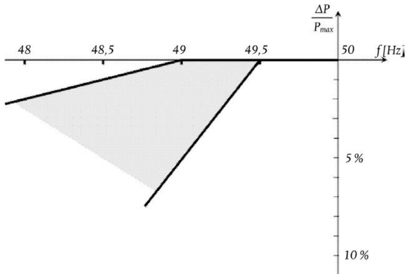
Maximum power capability reduction with falling frequency
