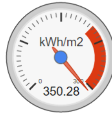
Primary energy
