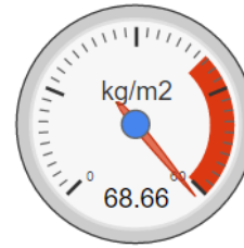
CO 2 emissions
