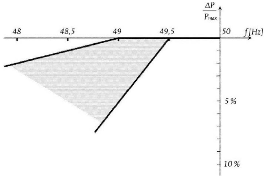
Figure 39 - Admissible active power reduction characteristic
