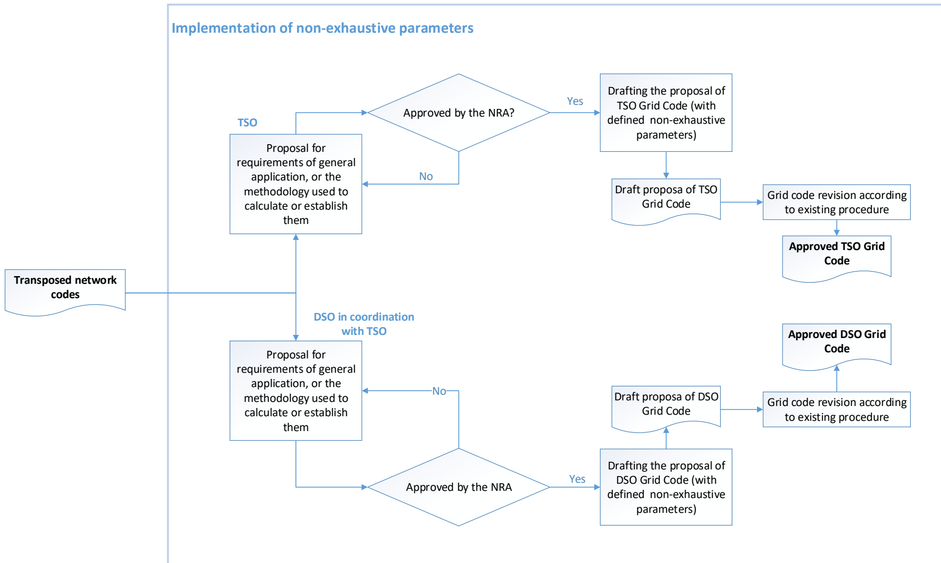
Figure 85 - Implementation of non- exhaustive parameters in existing grid code
