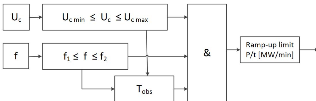
Figure 42 - Principle for automatic reconnection
