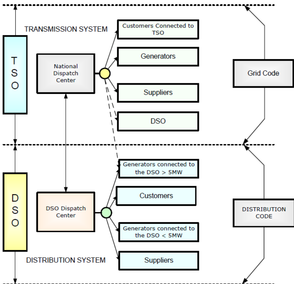
Figure 12 - Representation of TSO-DSO cooperation (data source [13])
