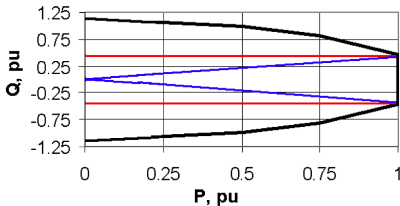
Figure 59 - Triangular, Rectangular and D-shape capability curve for 0.9 power factor at rated output (Source: [25] Figure 5)
