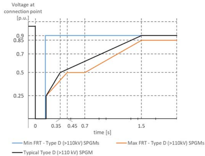
Figure 49 - Min and max possible FRT requirement, and typical response of type D SPGM connected at or above 110kV
