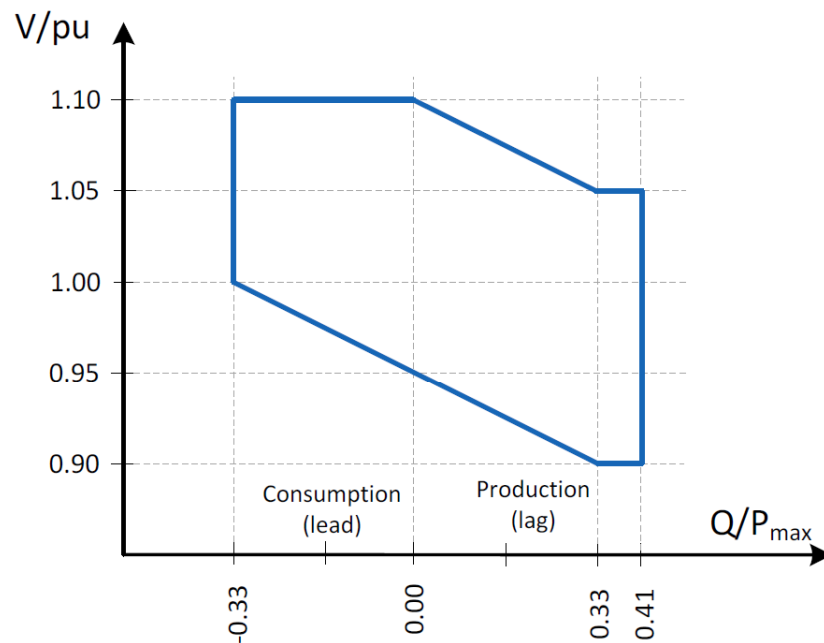
Figure 8: U-Q/P max -profile of a synchronous power-generating module. The diagram represents
