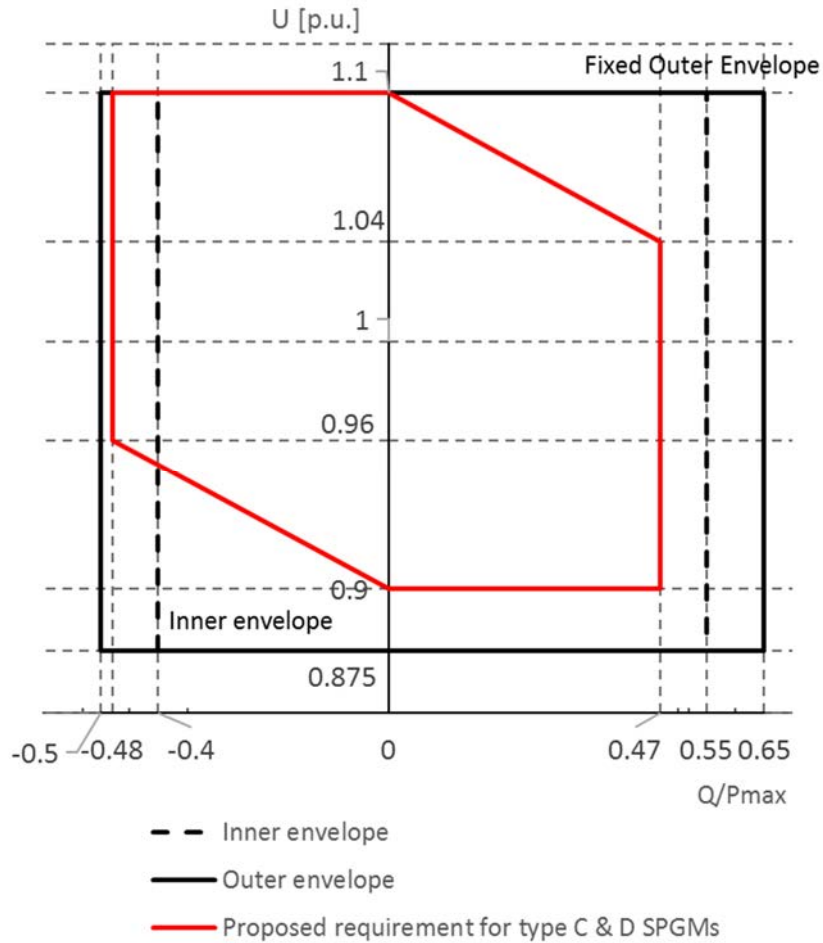
Figure 57 - Proposed U-Q/Pmax requirement for type C and D SPGMs
