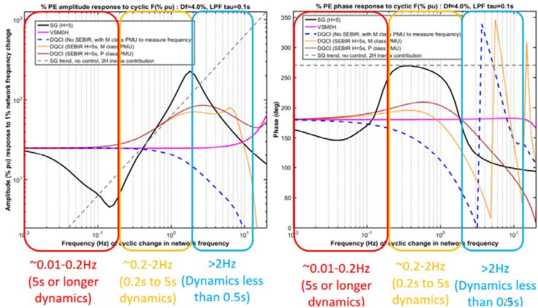
Figure 65 - Response of DQCI SEBIR controlled converters compared to SPGM's inertial response (Source: [17] Figure 2)
