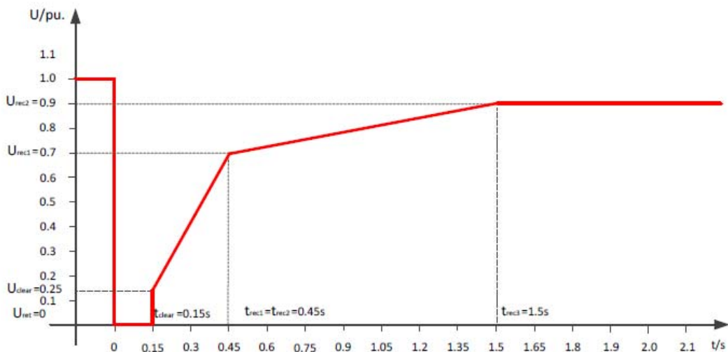
Figure 6: Fault-ride-through profile of a synchronous power-generating module connected in transmission network. The diagram represents the limit of a voltage-against-time profile of the voltage at the connection point, expressed as the ratio of its actual value and its reference 1 pu value before, during and after a fault. U_{ret} is the retained voltage at the connection point during a fault, t_{clear} is the instant when the fault has been cleared. U_{rec1} , U_{rec2} , t_{rec1} , t_{rec2} and t_{rec3} specify certain points of lower limits of voltage recovery and relevant times after fault clearance.
