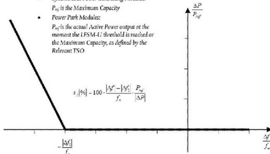
Figure 38 - LFSM-U characteristic
