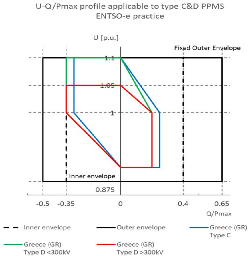
Figure 82– Reactive power capability requirement applicable to type C & D PPMS implemented in Greece
