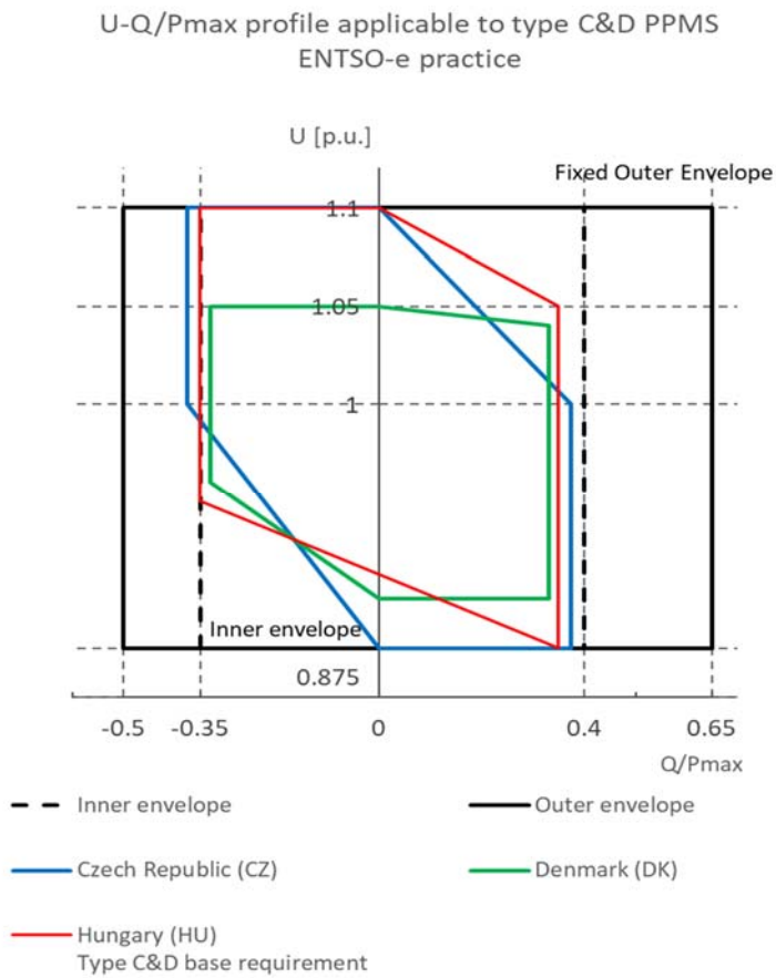
Figure 81– Reactive power capability requirement applicable to type C & D PPMS implemented in Czech Republic, Denmark and Hungary
