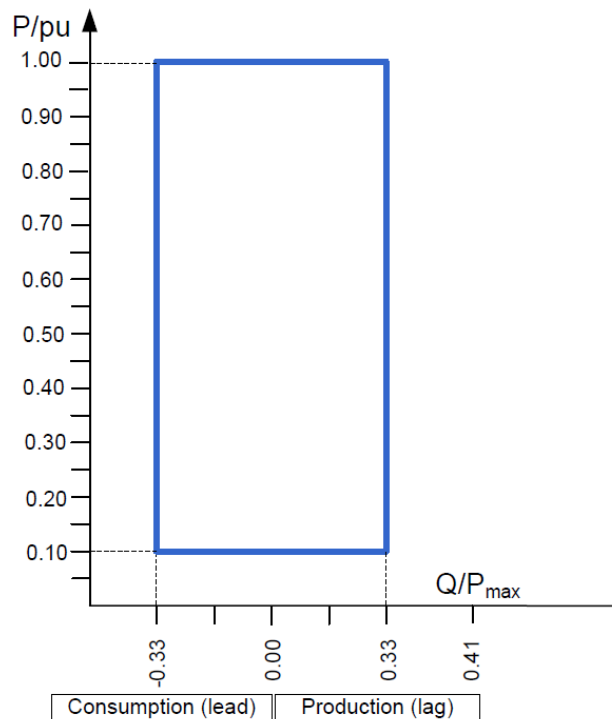
Figure 10: P-Q/P max -profile of a power park module with capacity ≥5MW. The diagram represents boundaries of a P-Q/P max -profile at the connection point by the active power, expressed by the ratio of its actual value and the maximum capacity pu, against the ratio of the reactive power (Q) and the maximum capacity (P max ).
