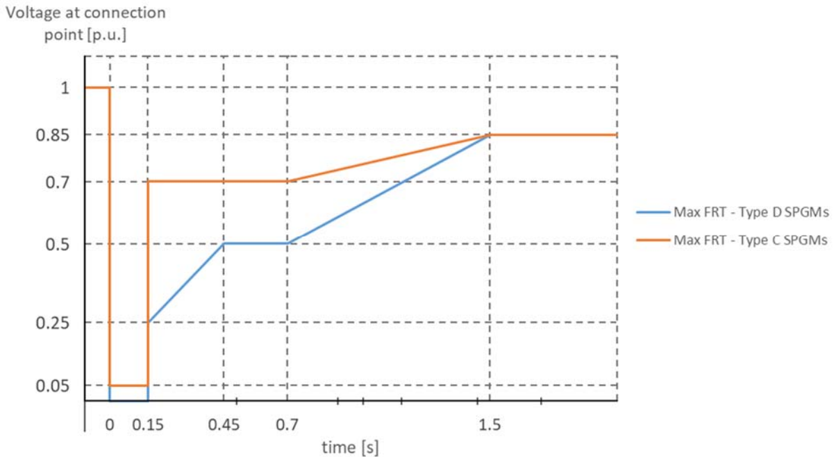
Figure 25 - Maximum FRT requirements for type C and D SPGMs
