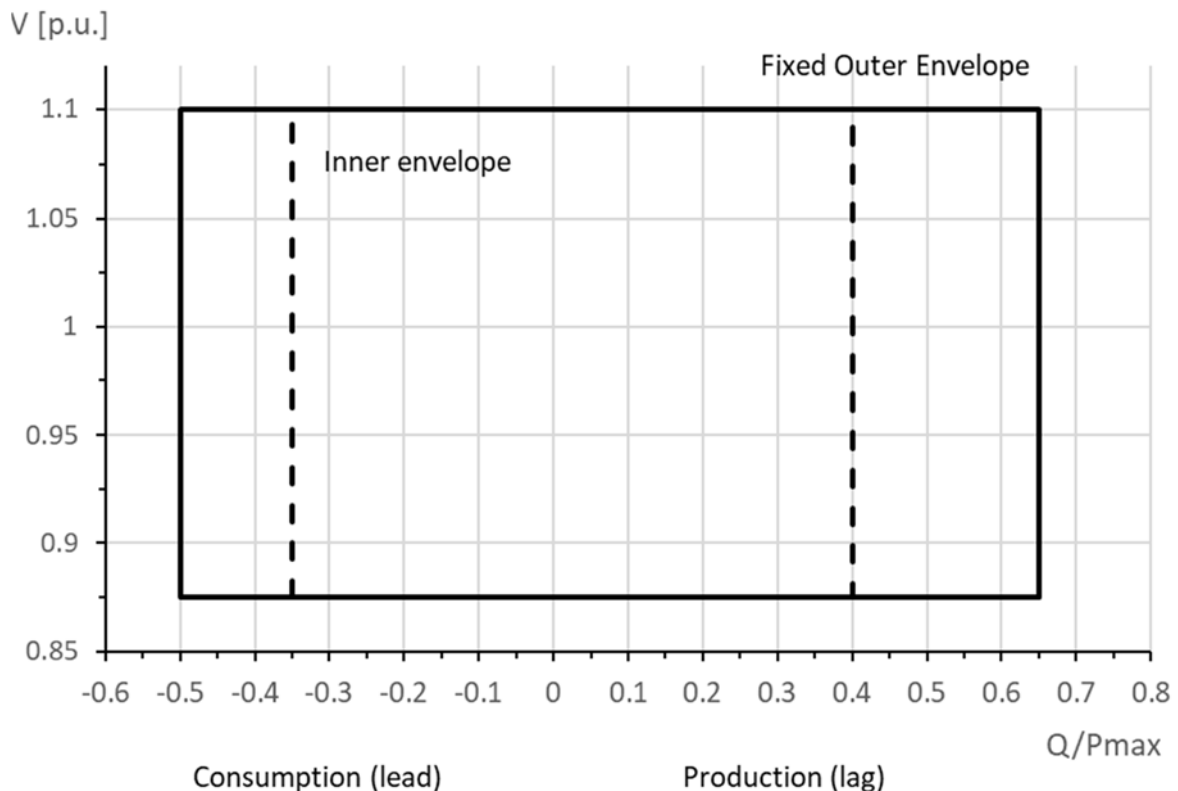
Figure 53 - U-Q/Pmax profile envelopes applicable to type C and D PPMs
