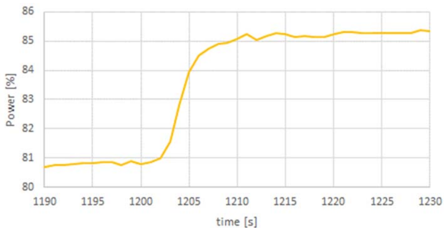
Figure 35 - FCR response of typical TPP
