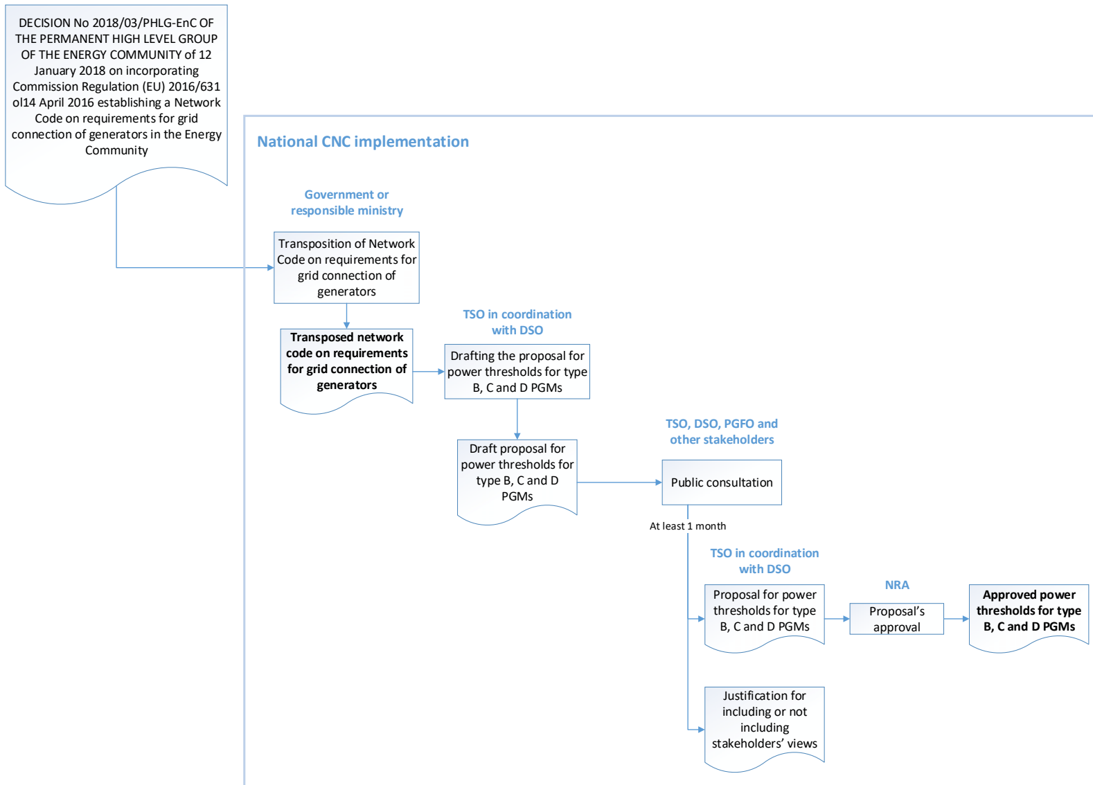
Figure 83 – Determination of significance process
