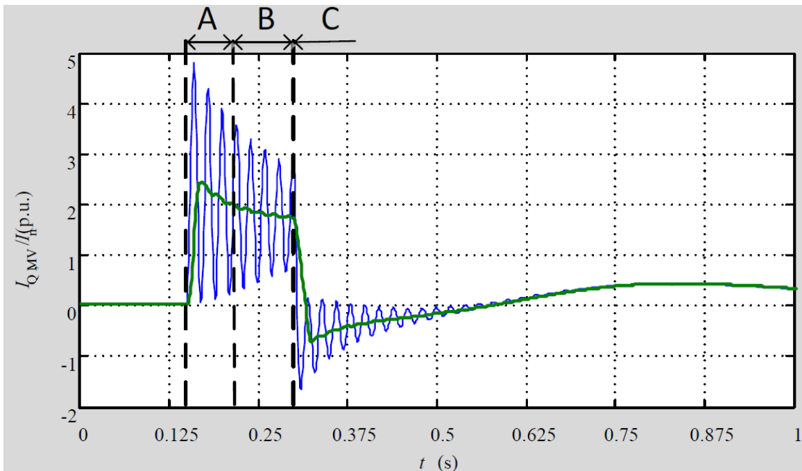
Figure 64 - Typical SPGM’s response to 3-phase fault (Data source: [20] Figure 1)
