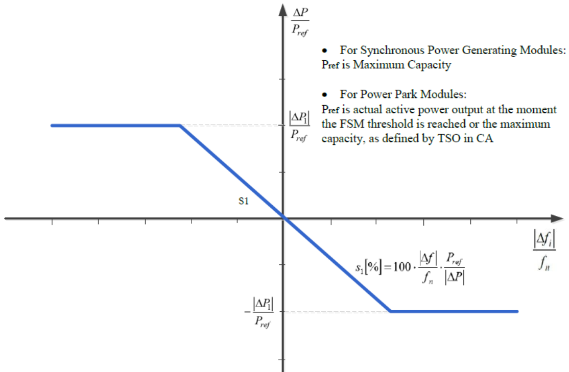
Figure 16 - FSM requirement (Connection Code Figure 4)
