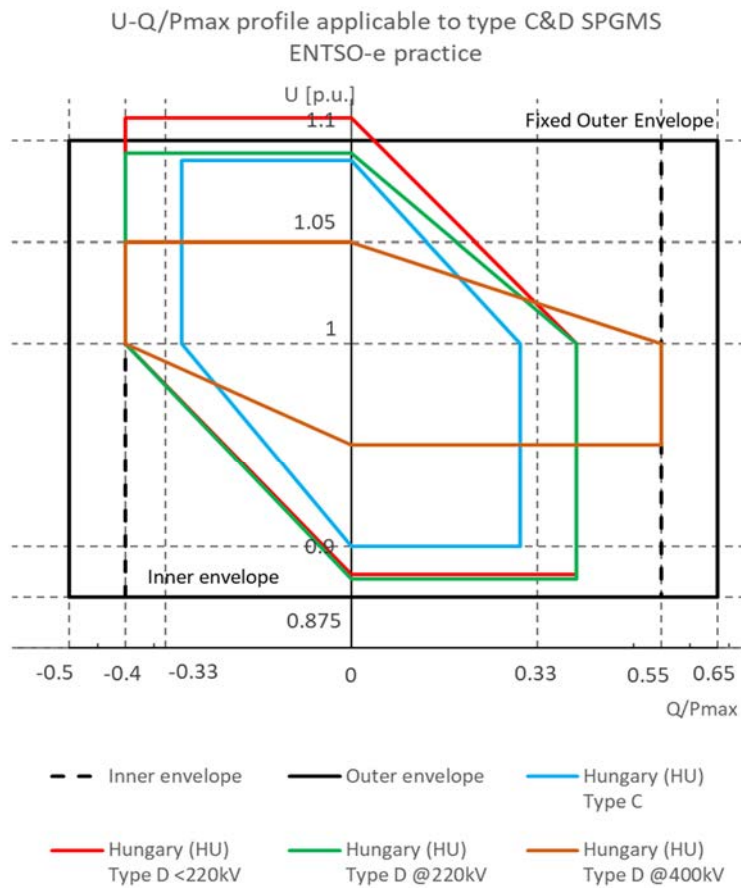
Figure 79– Reactive power capability requirement applicable to type C & D SPGMS implemented in Hungary
