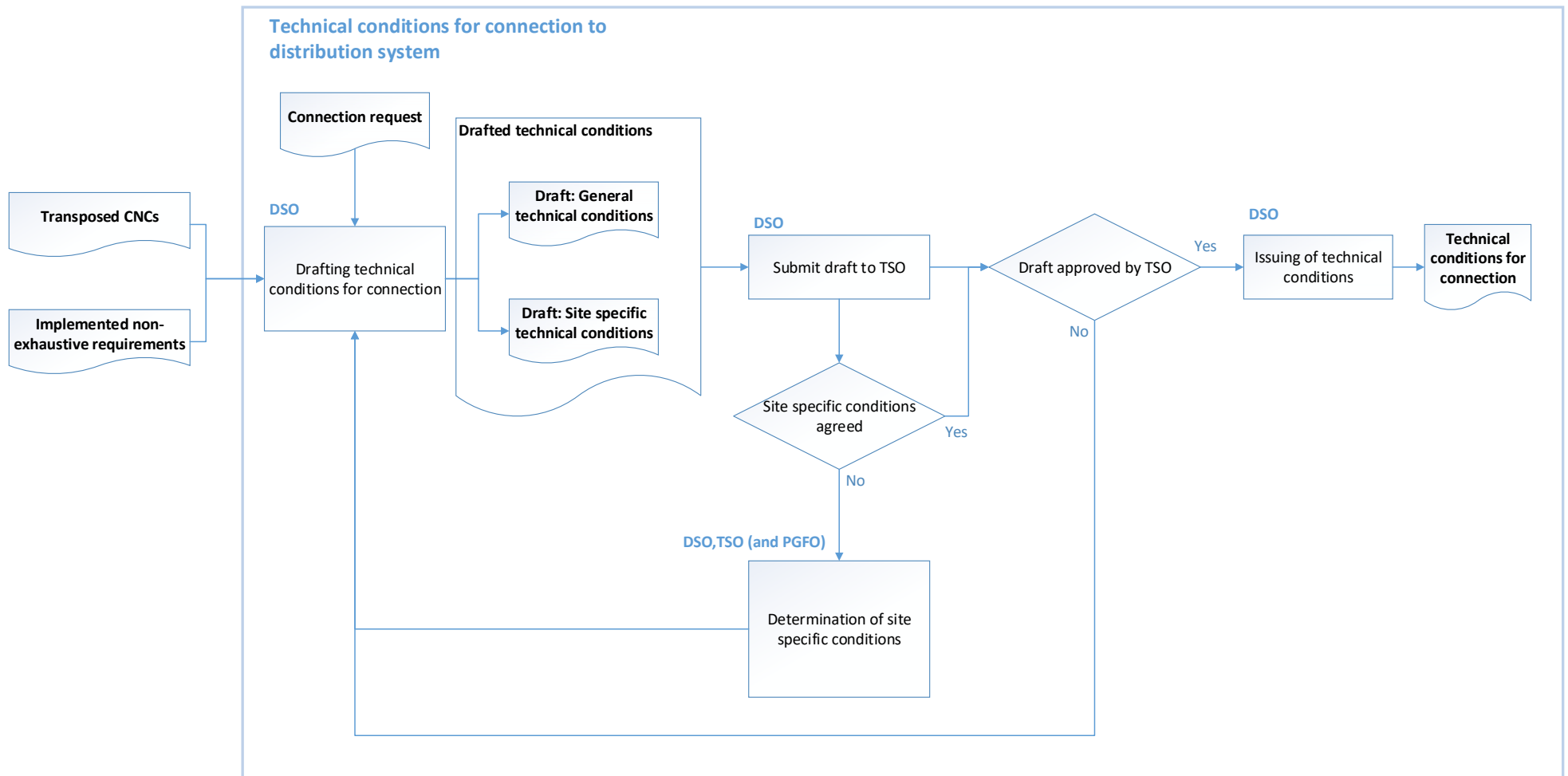
Figure 86 - DSO issues technical conditions for connection
