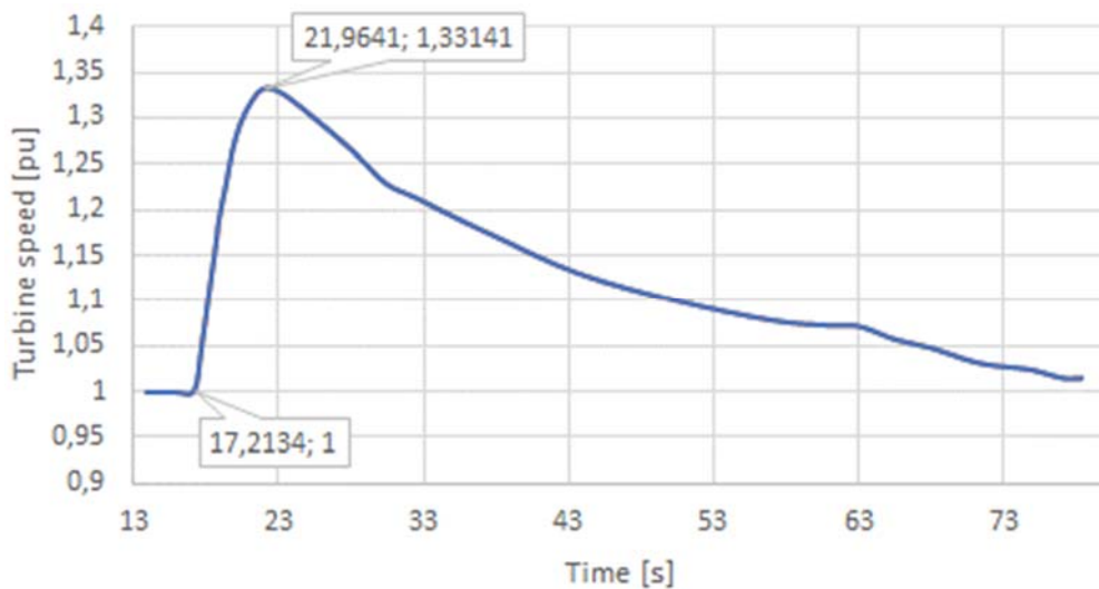
Figure 29 - Load rejection on typical HPP
