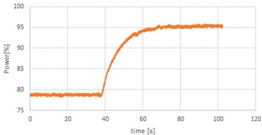
Figure 34 - FCR response of typical HPP
