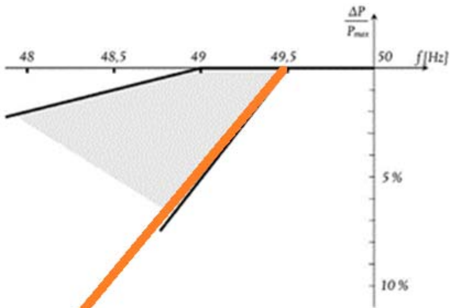
Figure 41 - Recommendation for parameter Admissible active power reduction from max. output with falling frequency
