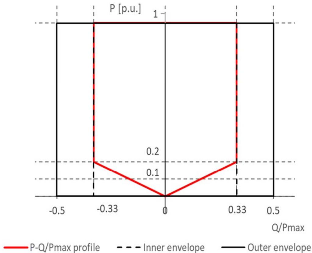
Figure 61 - Proposed P-Q/Pmax characteristics for PPMs Voltage/Reactive Power Control
