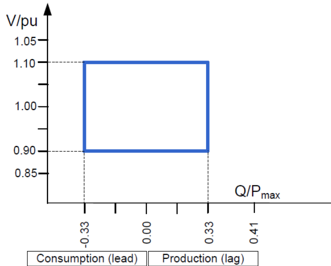
Figure 9: U-Q/P max -profile of a Power Park module with capacity ≥5MW. The diagram represents boundaries of a U-Q/P max -profile by the voltage at the connection point, expressed by the ratio of its actual value and it's the reference 1 pu value, against the ratio of the reactive power (Q) and the maximum capacity (P max ).
