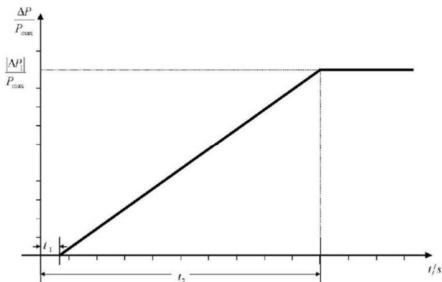
Figure 33 - FCR response characteristic
