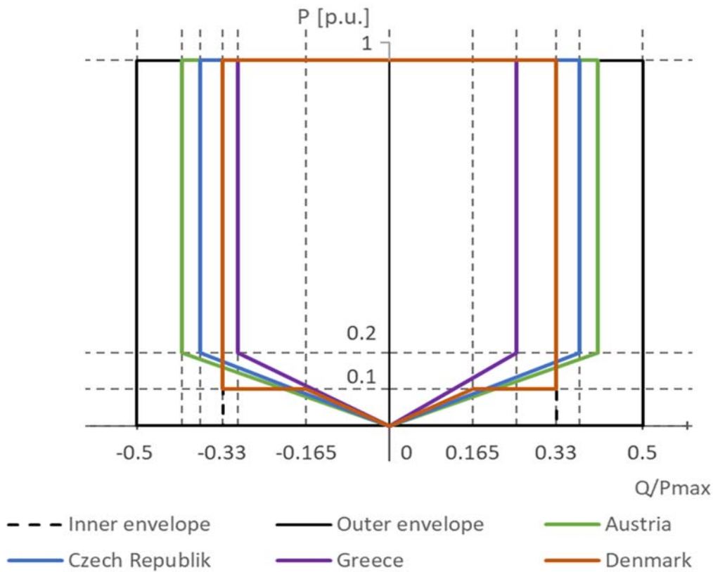
Figure 60 - Maximum size and position of P-Q/Pmax request and some of the requirements implemented in EU countries
