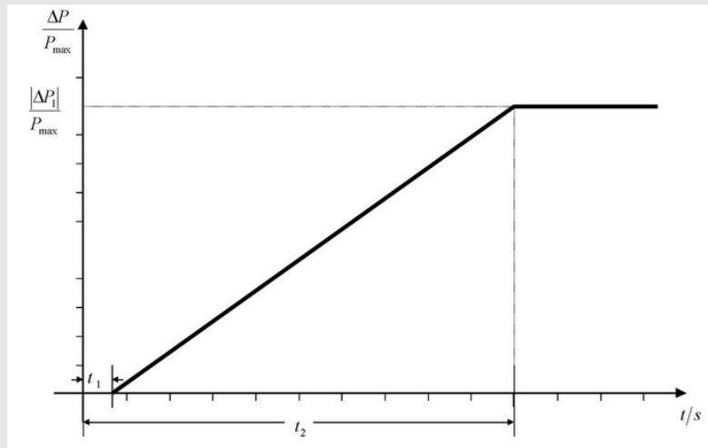
Figure 3- Active power frequency response capability ([1] Figure 6)
