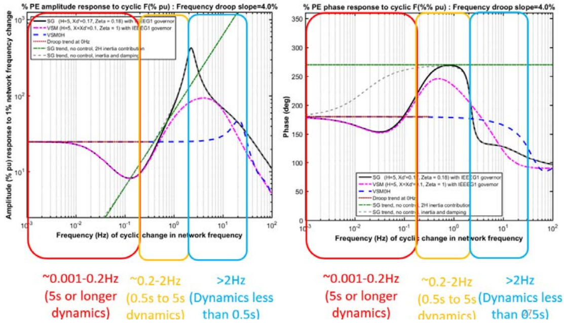
Figure 66 - Response of VSM controlled converters compared to SPGM's inertial response (Source: [17] Figure 1)
